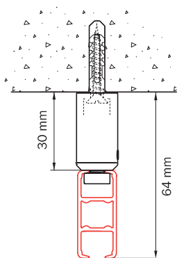
ceiling mounting with mini suspension hanger 4254
