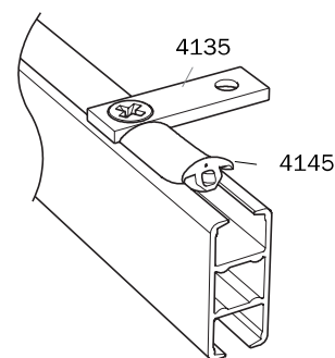
ceiling mounting with ceiling bracket 4135 and dust cover 4145 to seal the gap
